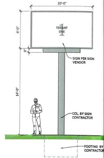
FREE STANDING SIGN SCALE: 1/4" = 1'-0"
