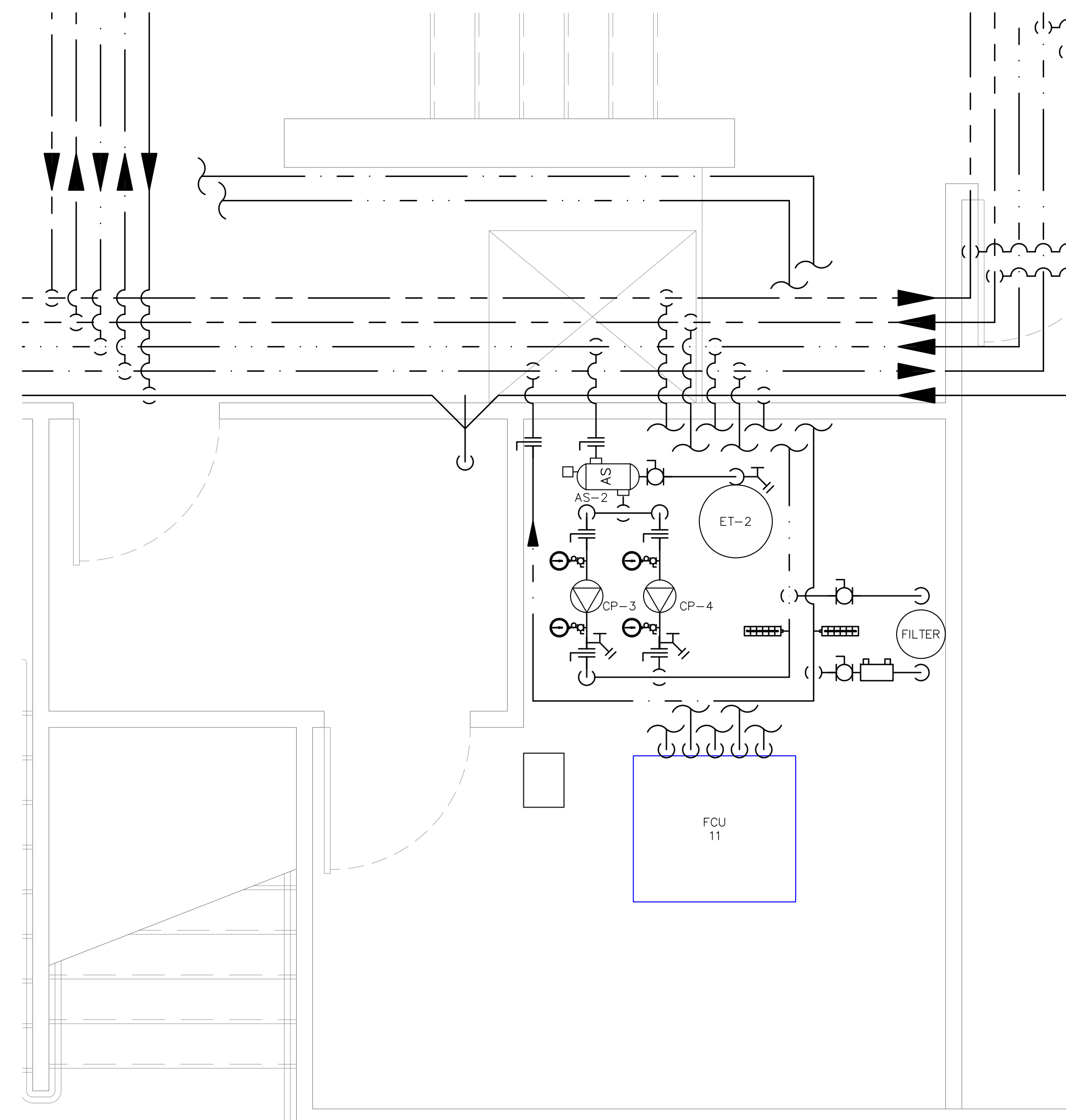
2 ENLARGED CHILLER ROOM PLAN M-3 1/2"=1'-0"
